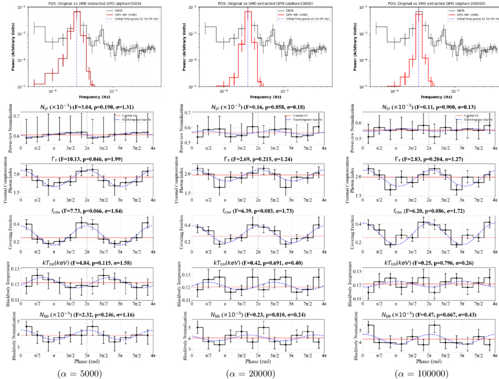
Figure 8. from Wen-Zhong Li et al 2026 Astrophys. J. Lett. 1005 doi:10.3847/2041-8213/ae7106 https://dx.doi.org/10.3847/2041-8213/ae7106 © 2026. The Author(s). Published by the American Astronomical Society.
