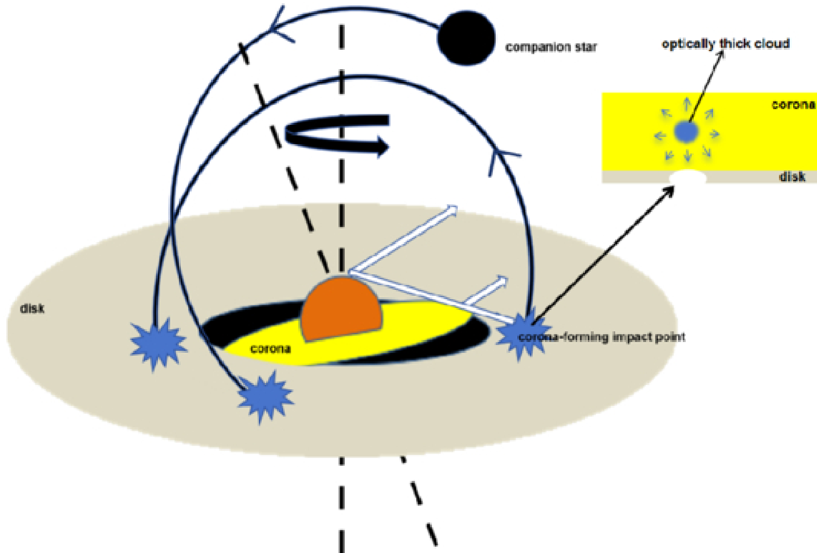
Figure 7. from Wen-Zhong Li et al 2026 Astrophys. J. Lett. 1005 doi:10.3847/2041-8213/ae7106 https://dx.doi.org/10.3847/2041-8213/ae7106 © 2026. The Author(s). Published by the American Astronomical Society.
