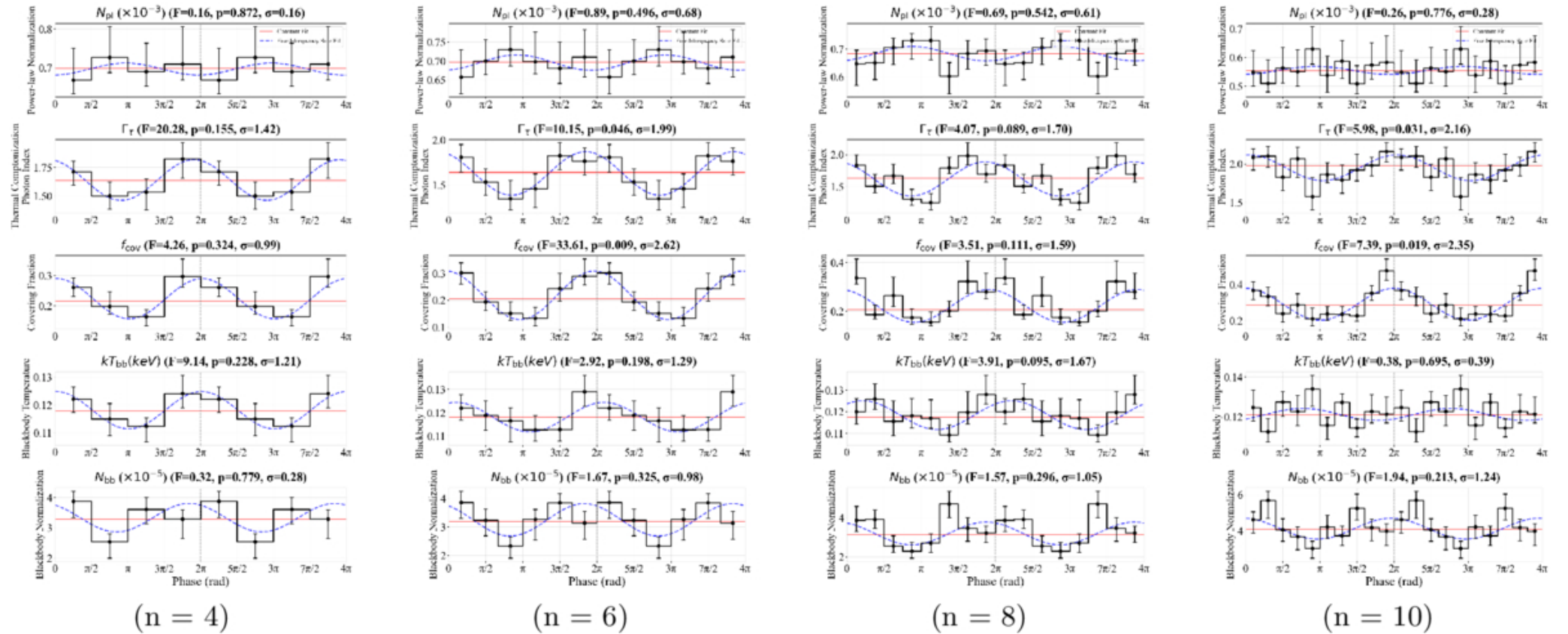
Figure 12. from Wen-Zhong Li et al 2026 Astrophys. J. Lett. 1005 doi:10.3847/2041-8213/ae7106 https://dx.doi.org/10.3847/2041-8213/ae7106 © 2026. The Author(s). Published by the American Astronomical Society.
