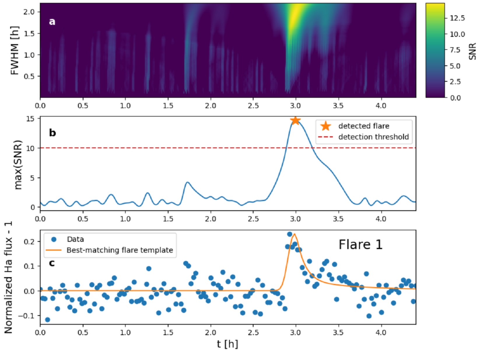
Figure 5. from Valeriy Vasilyev et al 2026 Astrophys. J. Lett. 1004 doi:10.3847/2041-8213/ae7078 https://dx.doi.org/10.3847/2041-8213/ae7078 © 2026. The Author(s). Published by the American Astronomical Society.
