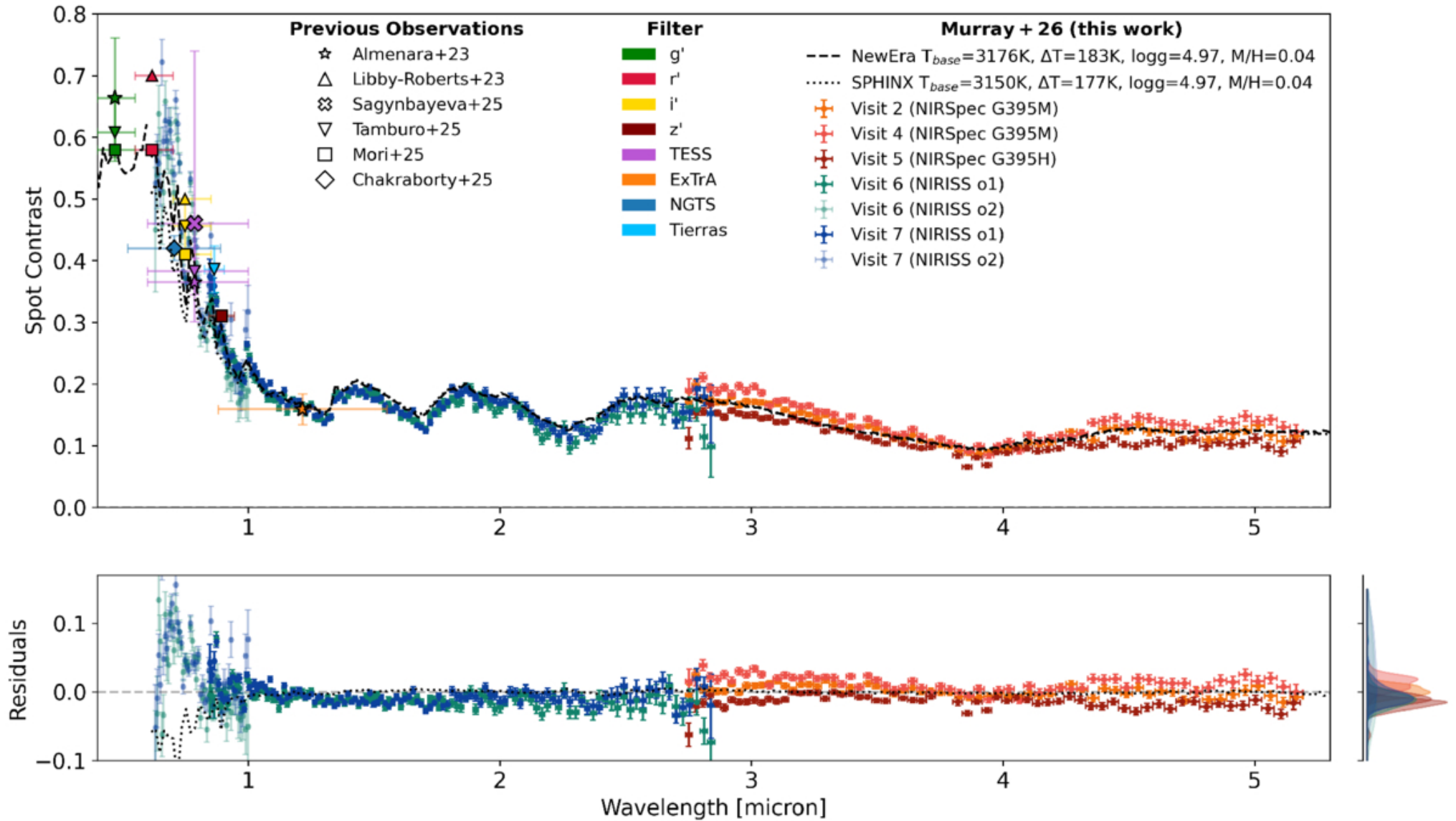
Figure 7. from C. A. Murray et al 2026 Astrophys. J. Lett. 1003 doi:10.3847/2041-8213/ae6fb6 https://dx.doi.org/10.3847/2041-8213/ae6fb6 © 2026. The Author(s). Published by the American Astronomical Society.
