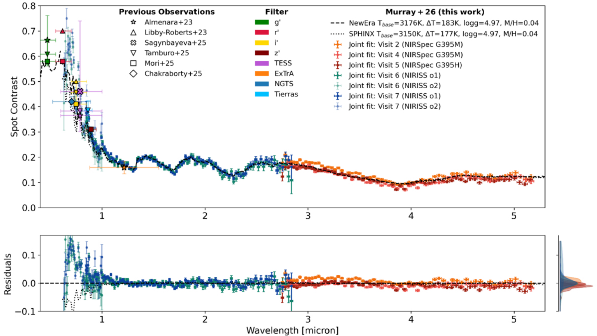
Figure 5. from C. A. Murray et al 2026 Astrophys. J. Lett. 1003 doi:10.3847/2041-8213/ae6fb6 https://dx.doi.org/10.3847/2041-8213/ae6fb6 © 2026. The Author(s). Published by the American Astronomical Society.
