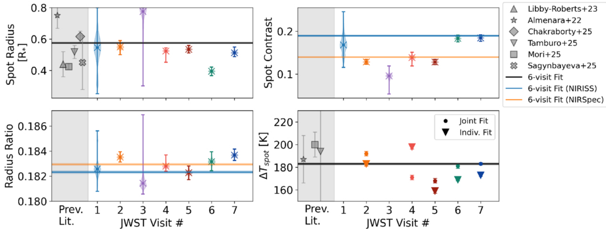
Figure 4. from C. A. Murray et al 2026 Astrophys. J. Lett. 1003 doi:10.3847/2041-8213/ae6fb6 https://dx.doi.org/10.3847/2041-8213/ae6fb6 © 2026. The Author(s). Published by the American Astronomical Society.
