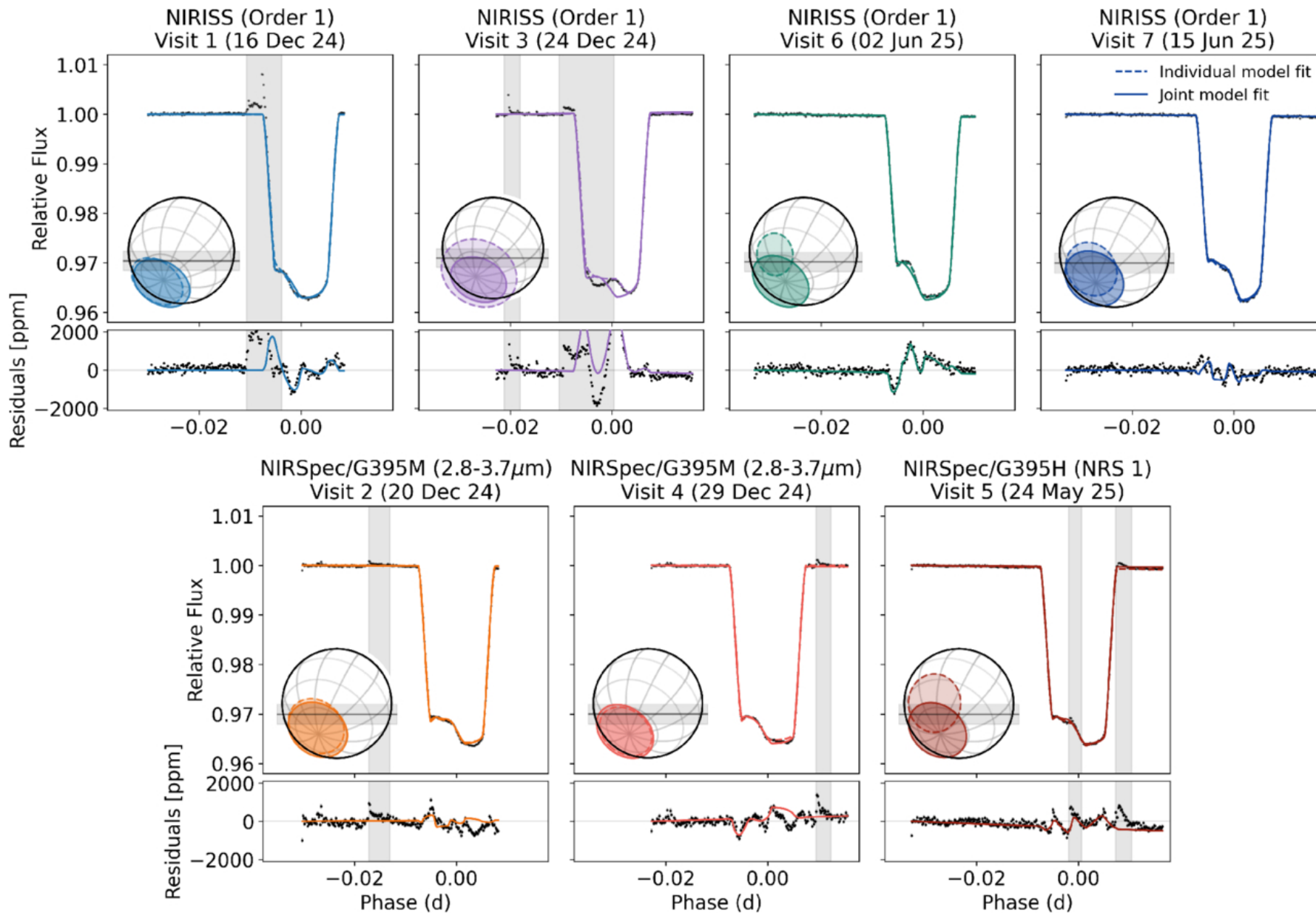
Figure 2. from C. A. Murray et al 2026 Astrophys. J. Lett. 1003 doi:10.3847/2041-8213/ae6fb6 https://dx.doi.org/10.3847/2041-8213/ae6fb6 © 2026. The Author(s). Published by the American Astronomical Society.
