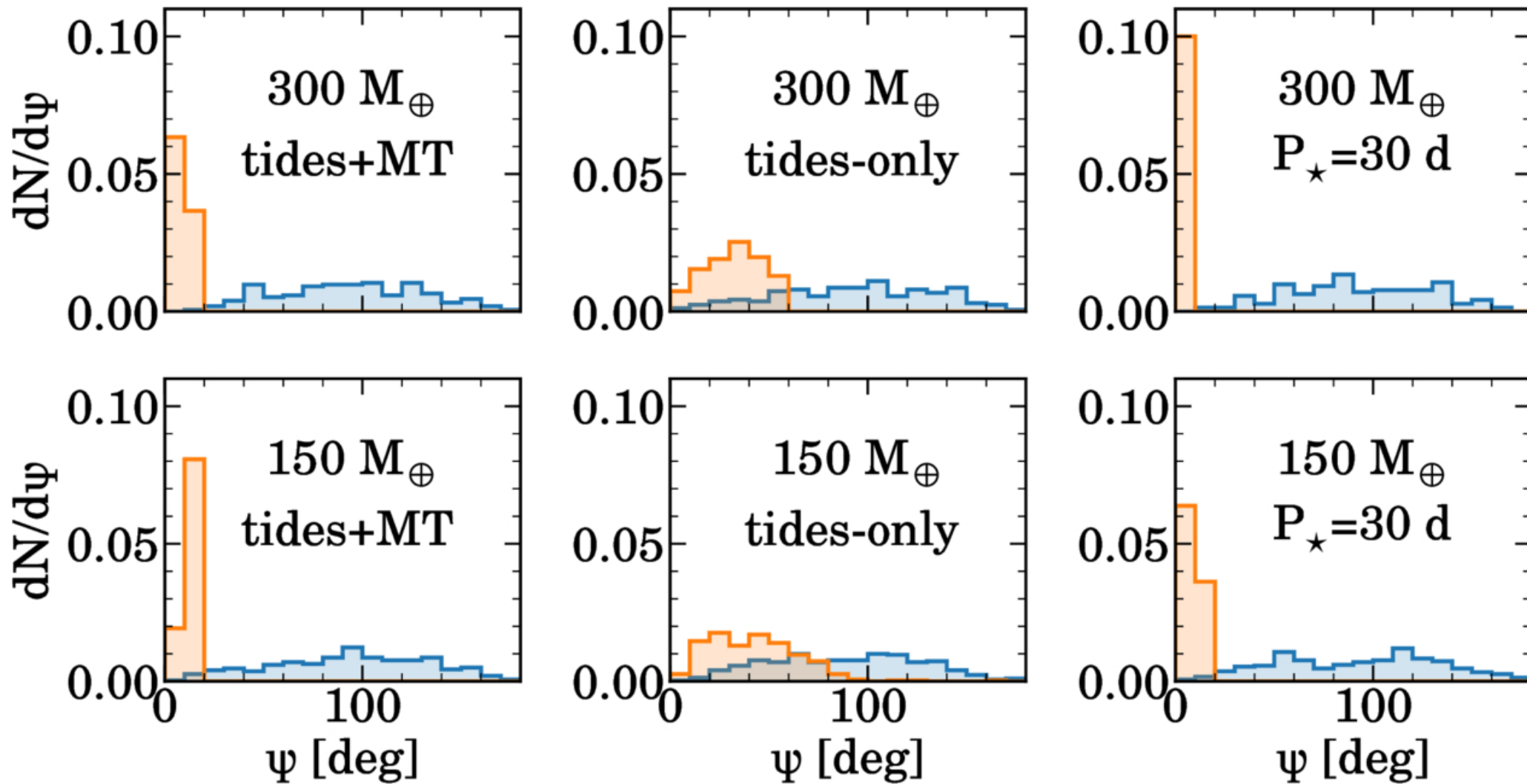
Figure 5. from Tim Hallatt et al 2026 Astrophys. J. Lett. 1005 doi:10.3847/2041-8213/ae6fb5 https://dx.doi.org/10.3847/2041-8213/ae6fb5 © 2026. The Author(s). Published by the American Astronomical Society.
