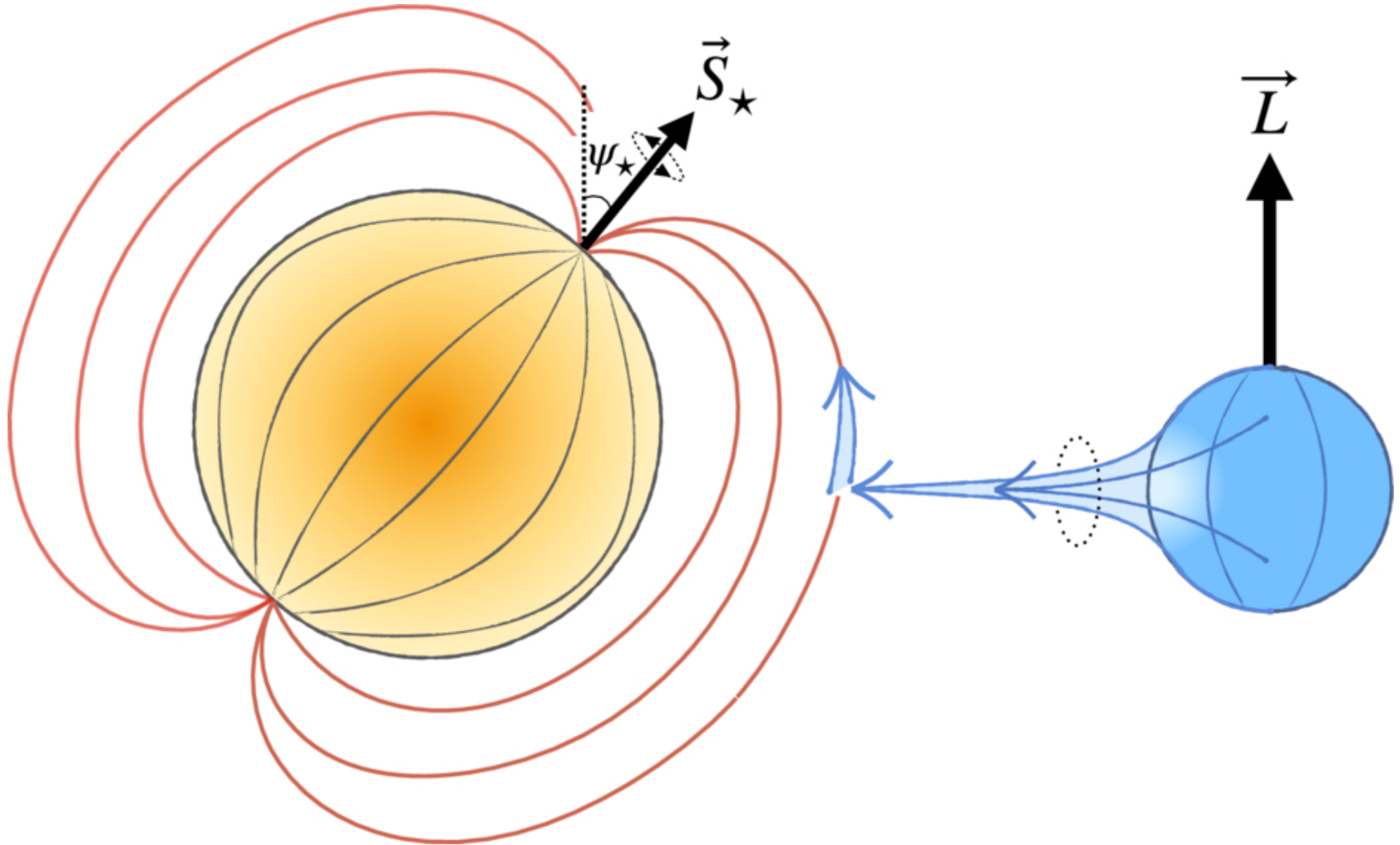
Figure 1. from Tim Hallatt et al 2026 Astrophys. J. Lett. 1005 doi:10.3847/2041-8213/ae6fb5 https://dx.doi.org/10.3847/2041-8213/ae6fb5 © 2026. The Author(s). Published by the American Astronomical Society.
