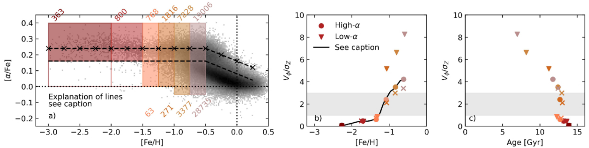
Figure 1. from Sofia Feltzing et al 2026 Astrophys. J. Lett. 1004 doi:10.3847/2041-8213/ae6f14 https://dx.doi.org/10.3847/2041-8213/ae6f14 © 2026. The Author(s). Published by the American Astronomical Society.
