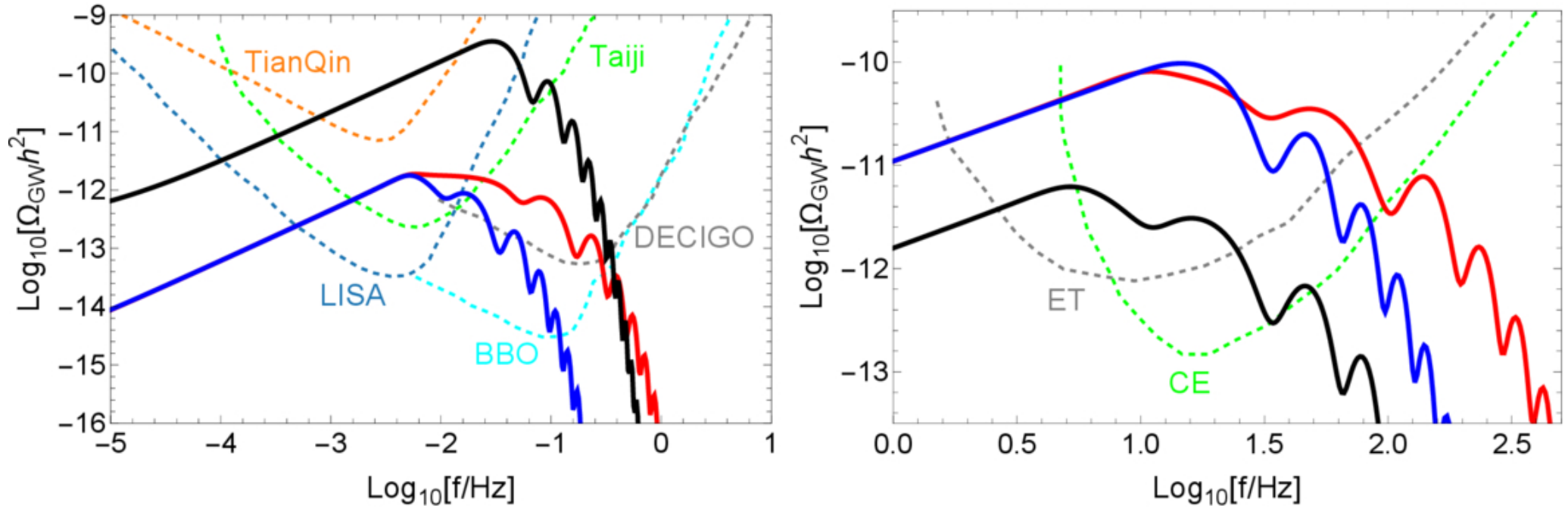
Figure 3. from Mian Zhu and Yi-Fu Cai 2026 Astrophys. J. Lett. 1004 doi:10.3847/2041-8213/ae6f10 https://dx.doi.org/10.3847/2041-8213/ae6f10 © 2026. The Author(s). Published by the American Astronomical Society.
