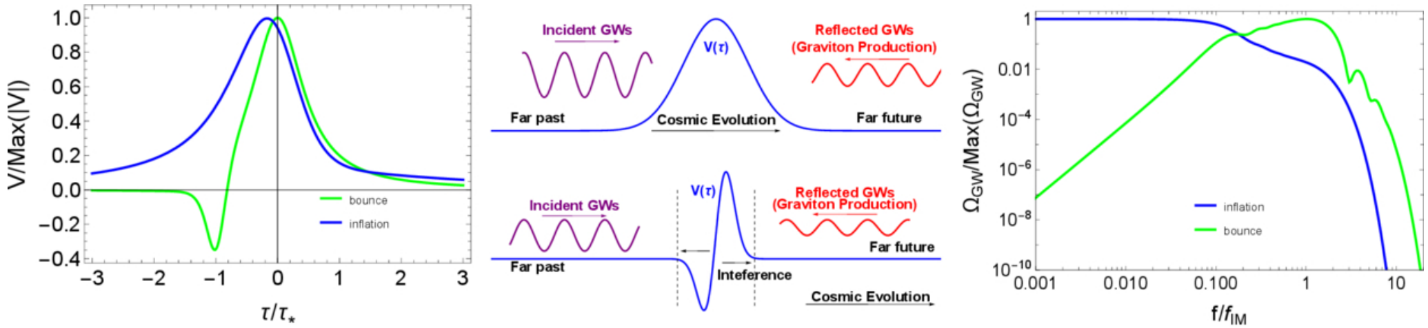
Figure 1. from Mian Zhu and Yi-Fu Cai 2026 Astrophys. J. Lett. 1004 doi:10.3847/2041-8213/ae6f10 https://dx.doi.org/10.3847/2041-8213/ae6f10 © 2026. The Author(s). Published by the American Astronomical Society.
