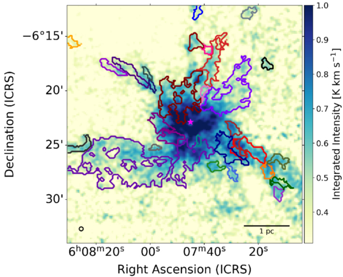
Figure 6. from Jihye Hwang et al 2026 Astrophys. J. Lett. 1004 doi:10.3847/2041-8213/ae6f0f https://dx.doi.org/10.3847/2041-8213/ae6f0f © 2026. The Author(s). Published by the American Astronomical Society.
