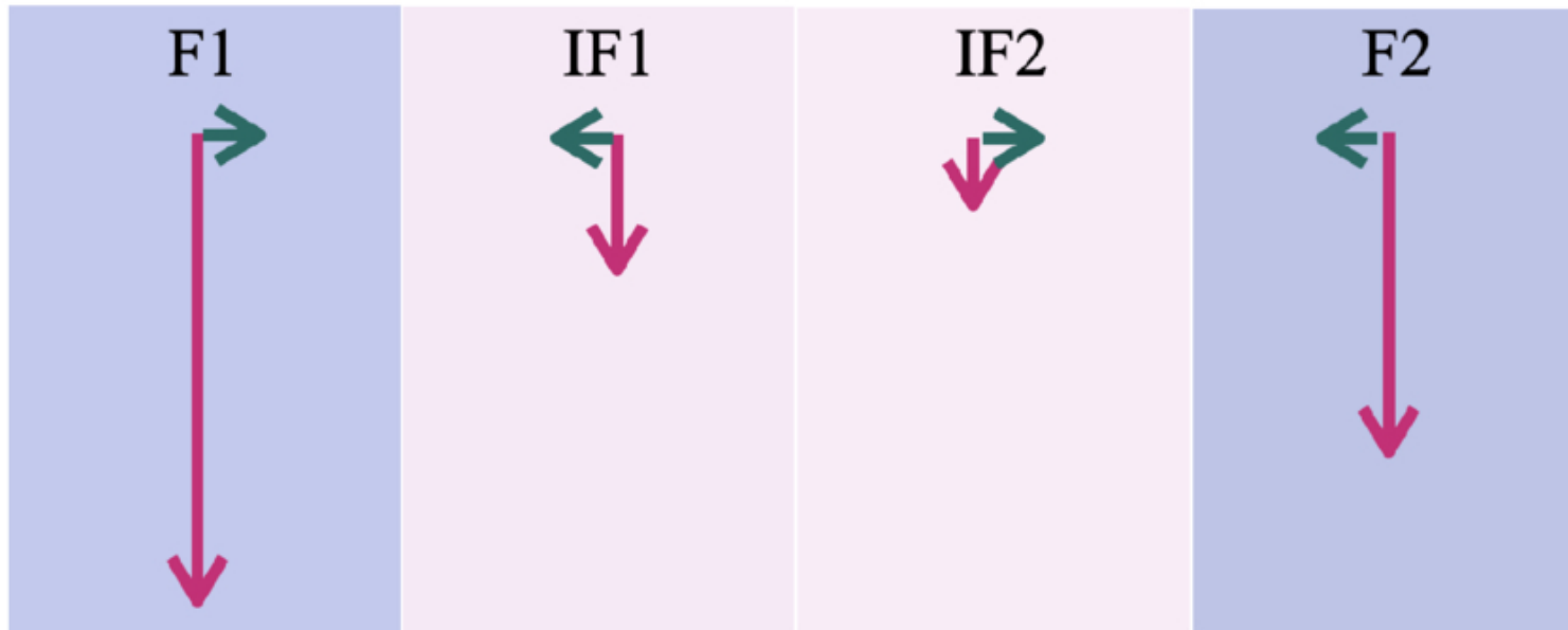
Figure 3. from Jihye Hwang et al 2026 Astrophys. J. Lett. 1004 doi:10.3847/2041-8213/ae6f0f https://dx.doi.org/10.3847/2041-8213/ae6f0f © 2026. The Author(s). Published by the American Astronomical Society.
