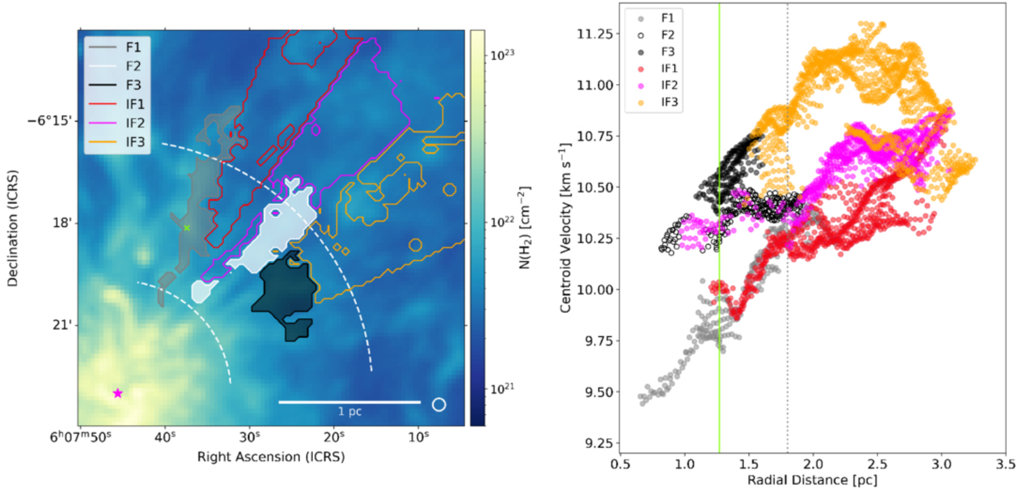
Figure 1. from Jihye Hwang et al 2026 Astrophys. J. Lett. 1004 doi:10.3847/2041-8213/ae6f0f https://dx.doi.org/10.3847/2041-8213/ae6f0f © 2026. The Author(s). Published by the American Astronomical Society.
