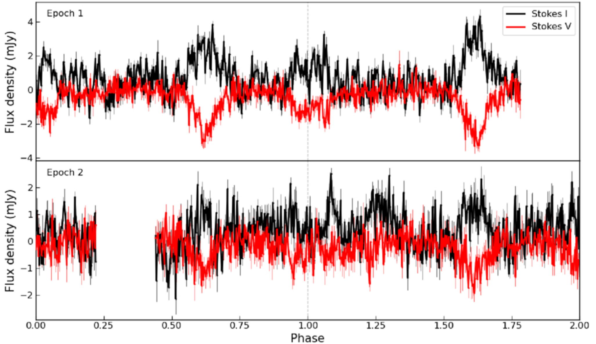
Figure 3. from Shouzhi Wang et al 2026 Astrophys. J. Lett. 1003 doi:10.3847/2041-8213/ae6ef6 https://dx.doi.org/10.3847/2041-8213/ae6ef6 © 2026. The Author(s). Published by the American Astronomical Society.
