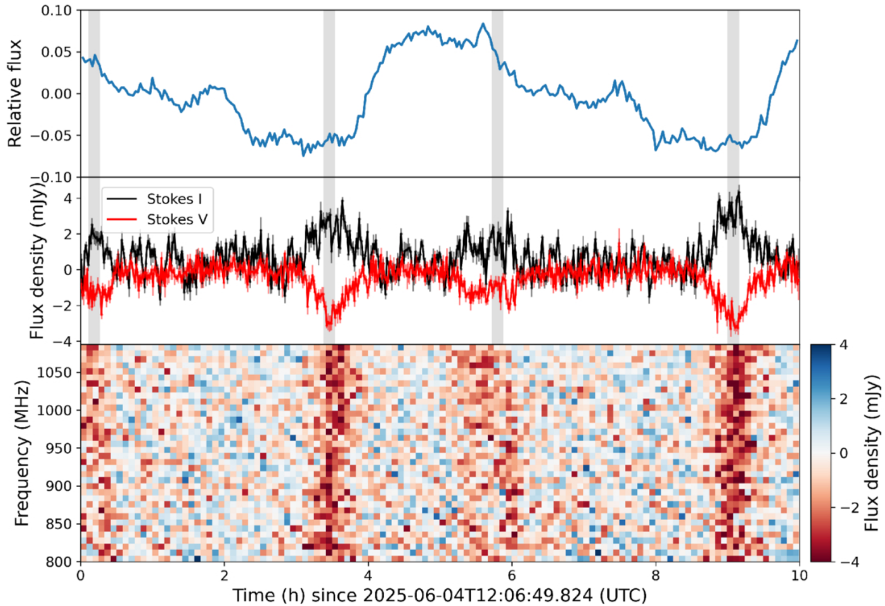
Figure 1. from Shouzhi Wang et al 2026 Astrophys. J. Lett. 1003 doi:10.3847/2041-8213/ae6ef6 https://dx.doi.org/10.3847/2041-8213/ae6ef6 © 2026. The Author(s). Published by the American Astronomical Society.
