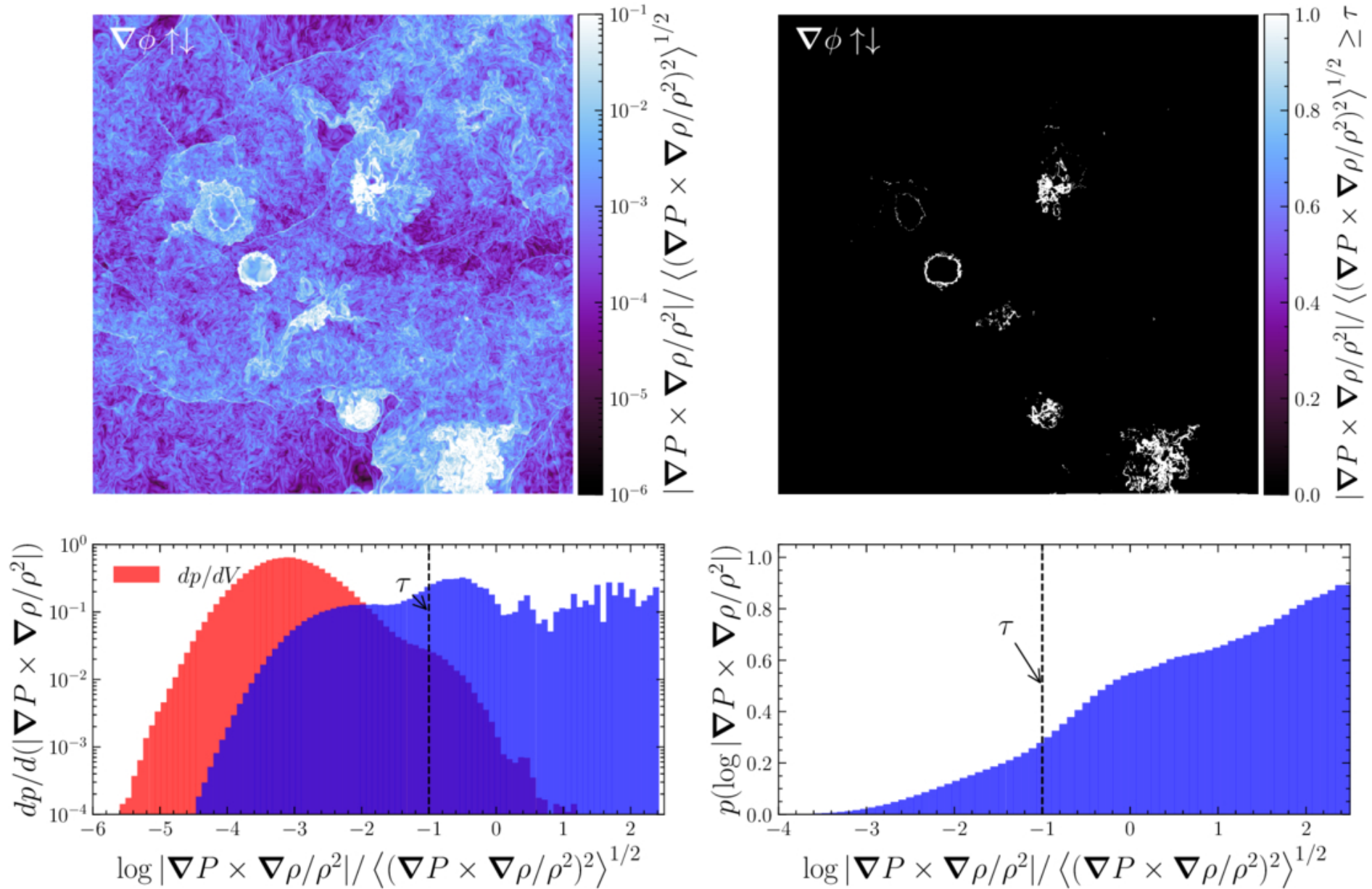
Figure 9. from James R. Beattie 2026 Astrophys. J. Lett. 1004 doi:10.3847/2041-8213/ae6eed https://dx.doi.org/10.3847/2041-8213/ae6eed © 2026. The Author(s). Published by the American Astronomical Society.
