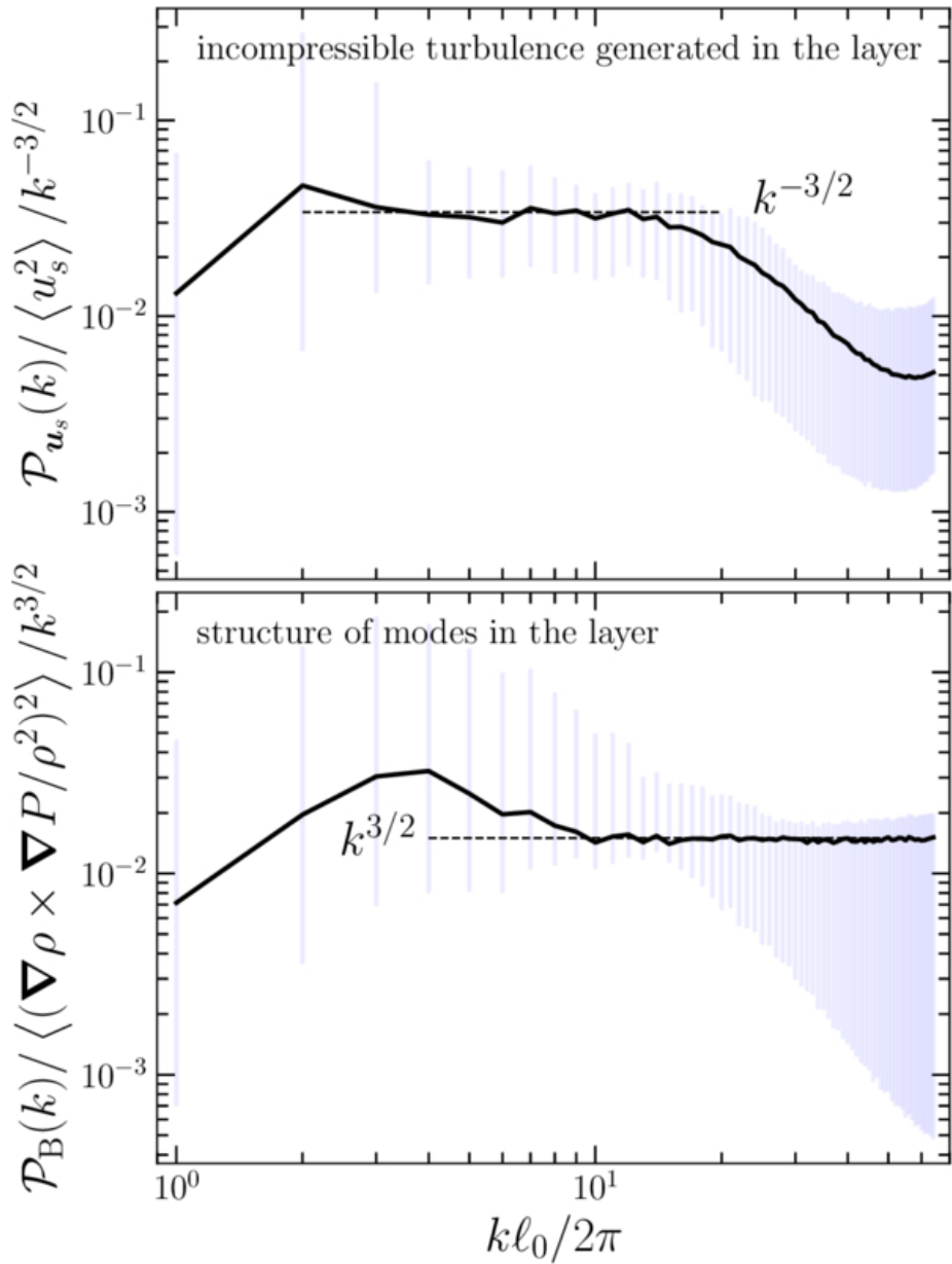
Figure 3. from James R. Beattie 2026 Astrophys. J. Lett. 1004 doi:10.3847/2041-8213/ae6eed https://dx.doi.org/10.3847/2041-8213/ae6eed © 2026. The Author(s). Published by the American Astronomical Society.
