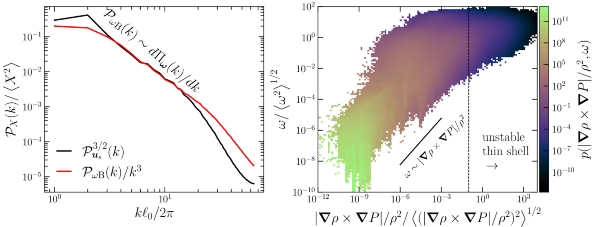
Figure 2. from James R. Beattie 2026 Astrophys. J. Lett. 1004 doi:10.3847/2041-8213/ae6eed https://dx.doi.org/10.3847/2041-8213/ae6eed © 2026. The Author(s). Published by the American Astronomical Society.
