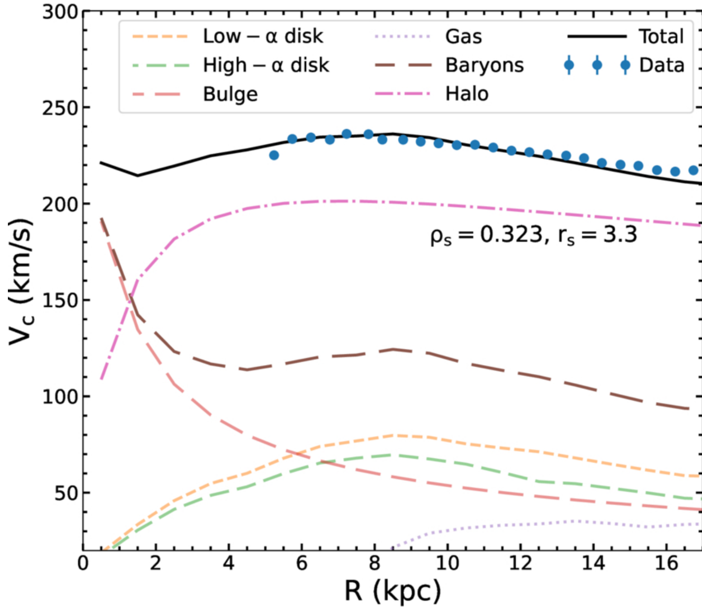
Figure 3. from Jianhui Lian et al 2026 Astrophys. J. Lett. 1003 doi:10.3847/2041-8213/ae6e40 https://dx.doi.org/10.3847/2041-8213/ae6e40 © 2026. The Author(s). Published by the American Astronomical Society.
