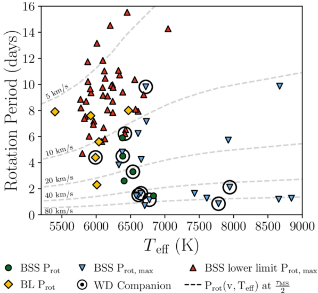
Figure 3. from Evan Linck and Robert D. Mathieu 2026 Astrophys. J. Lett. 1005 doi:10.3847/2041-8213/ae6e3d https://dx.doi.org/10.3847/2041-8213/ae6e3d © 2026. The Author(s). Published by the American Astronomical Society.
