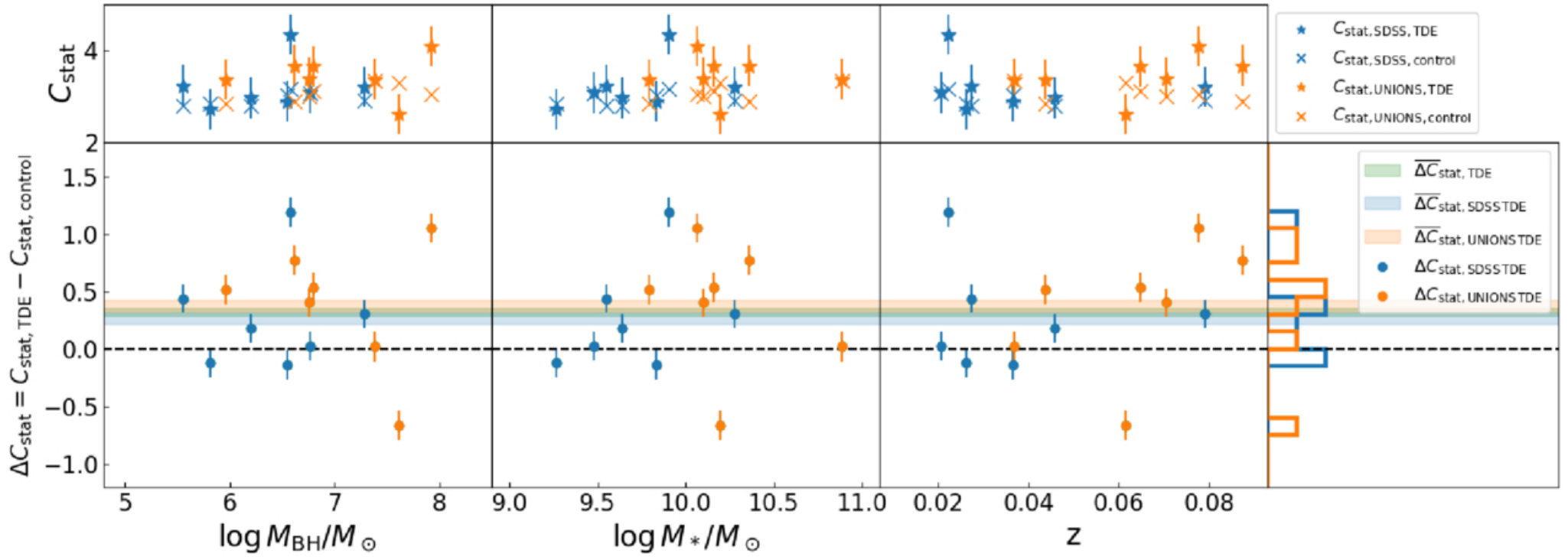
Figure 5. from Janet N.Y. Chang et al 2026 Astrophys. J. Lett. 1004 doi:10.3847/2041-8213/ae6db3 https://dx.doi.org/10.3847/2041-8213/ae6db3 © 2026. The Author(s). Published by the American Astronomical Society.
