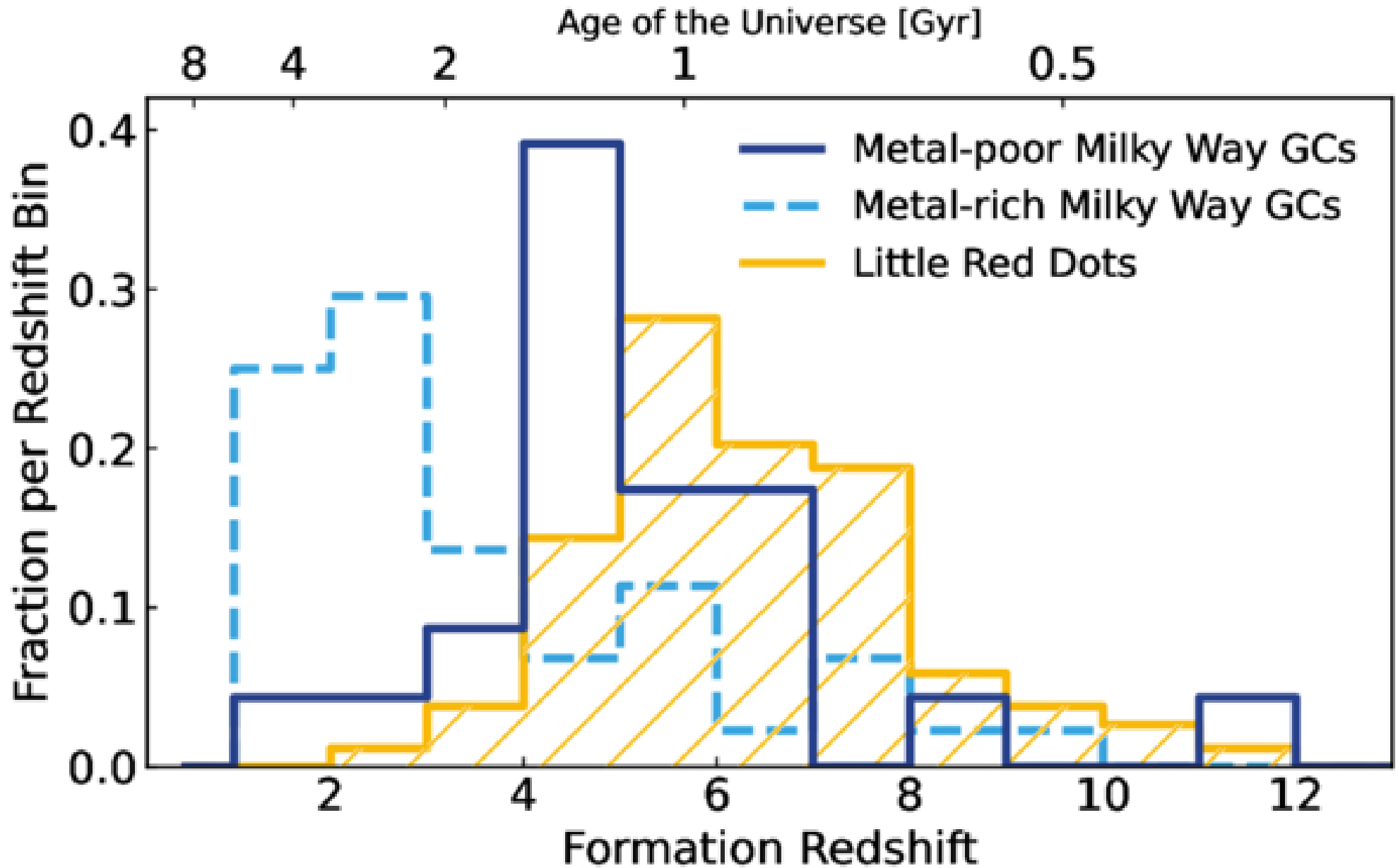
Figure 4. from John Chisholm et al 2026 Astrophys. J. Lett. 1004 doi:10.3847/2041-8213/ae6dae https://dx.doi.org/10.3847/2041-8213/ae6dae © 2026. The Author(s). Published by the American Astronomical Society.
