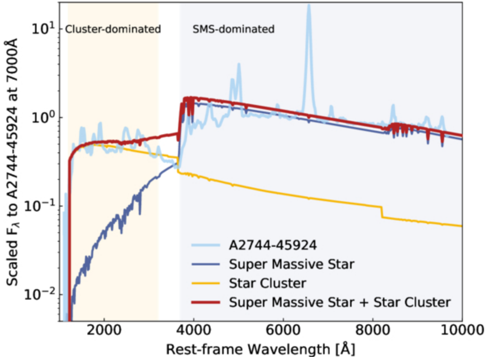
Figure 1. from John Chisholm et al 2026 Astrophys. J. Lett. 1004 doi:10.3847/2041-8213/ae6dae https://dx.doi.org/10.3847/2041-8213/ae6dae © 2026. The Author(s). Published by the American Astronomical Society.
