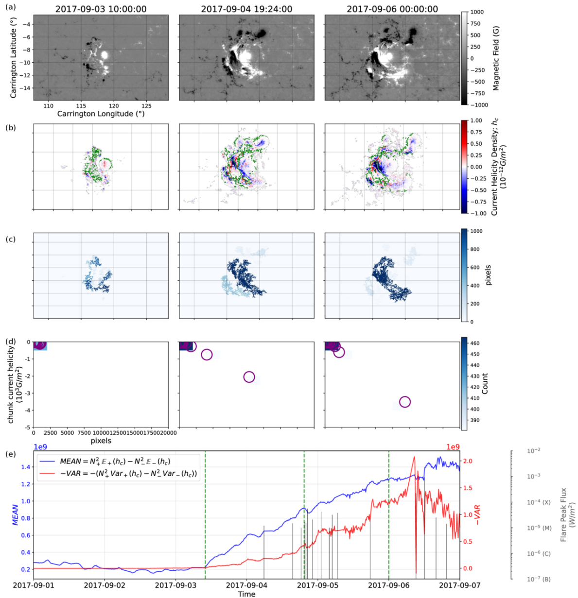
Figure 3. from Youngjae Kim et al 2026 Astrophys. J. Lett. 1005 doi:10.3847/2041-8213/ae6cf8 https://dx.doi.org/10.3847/2041-8213/ae6cf8 © 2026. The Author(s). Published by the American Astronomical Society.
