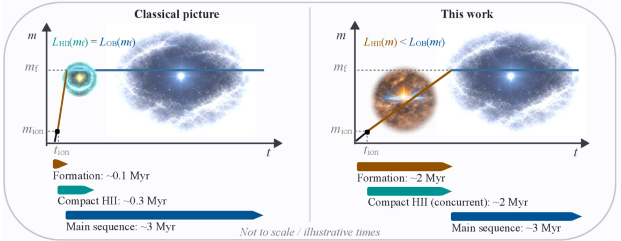
Figure 1. from Paolo Padoan and Mark Gieles 2026 Astrophys. J. Lett. 1003 doi:10.3847/2041-8213/ae6c23 https://dx.doi.org/10.3847/2041-8213/ae6c23 © 2026. The Author(s). Published by the American Astronomical Society.
