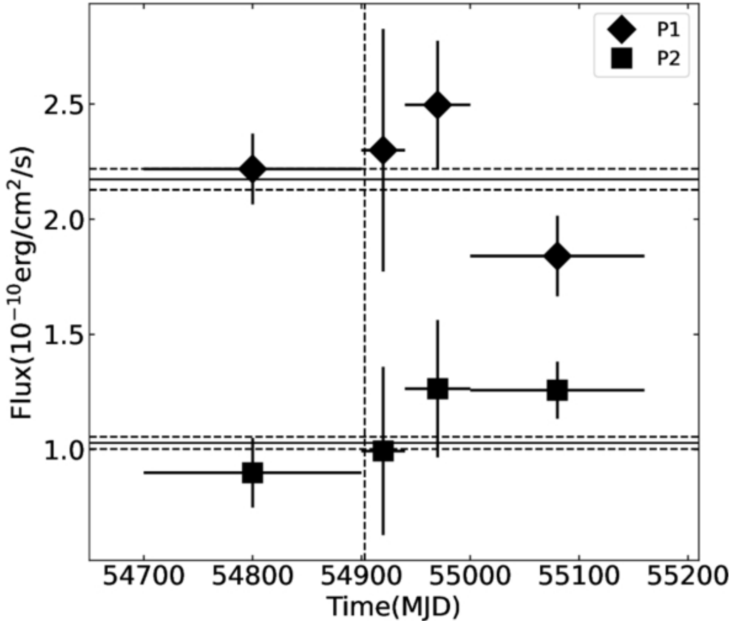
Figure 3. from Wen-Tao Ye et al 2026 Astrophys. J. Lett. 1003 doi:10.3847/2041-8213/ae6b6b https://dx.doi.org/10.3847/2041-8213/ae6b6b © 2026. The Author(s). Published by the American Astronomical Society.
