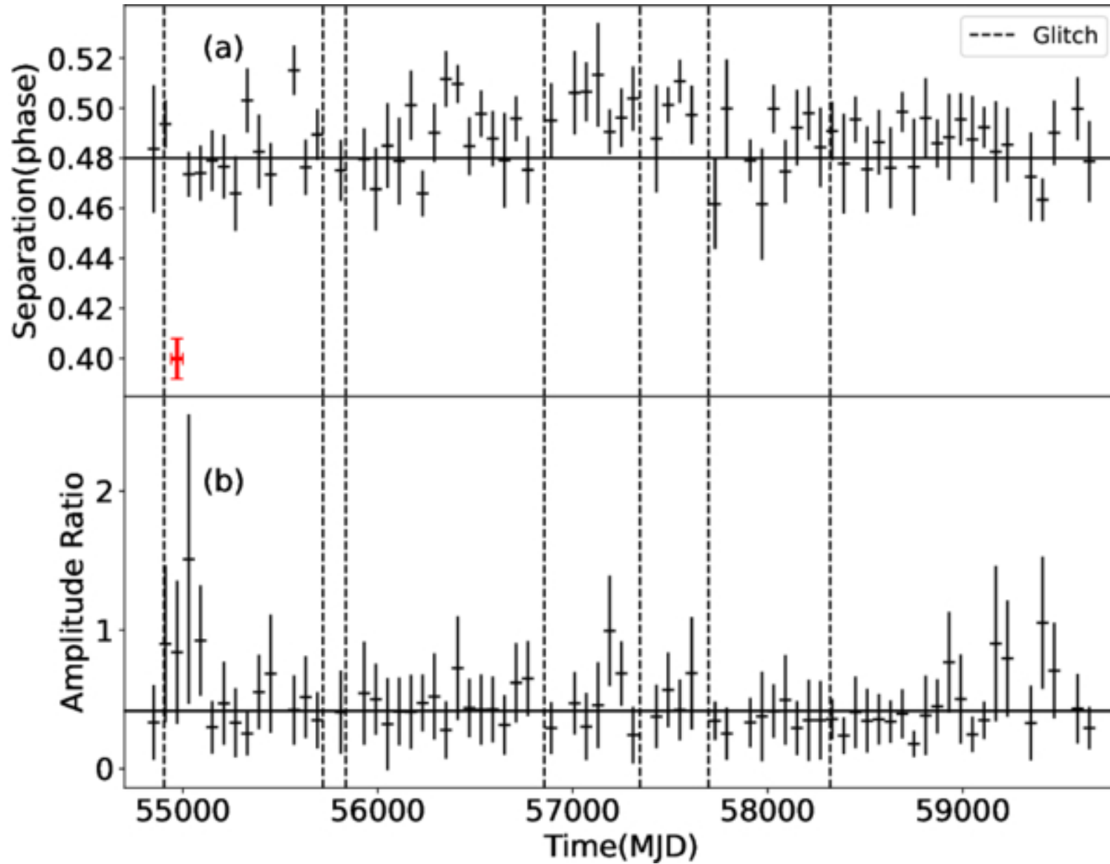
Figure 2. from Wen-Tao Ye et al 2026 Astrophys. J. Lett. 1003 doi:10.3847/2041-8213/ae6b6b https://dx.doi.org/10.3847/2041-8213/ae6b6b © 2026. The Author(s). Published by the American Astronomical Society.
