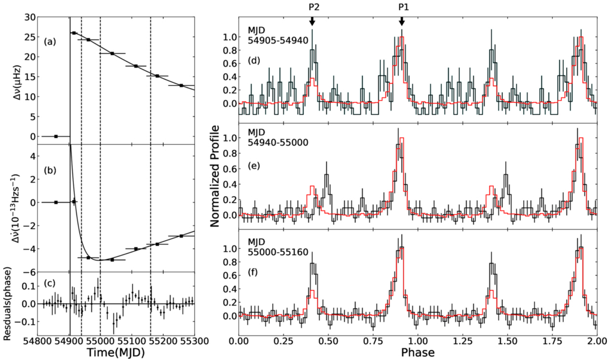
Figure 1. from Wen-Tao Ye et al 2026 Astrophys. J. Lett. 1003 doi:10.3847/2041-8213/ae6b6b https://dx.doi.org/10.3847/2041-8213/ae6b6b © 2026. The Author(s). Published by the American Astronomical Society.
