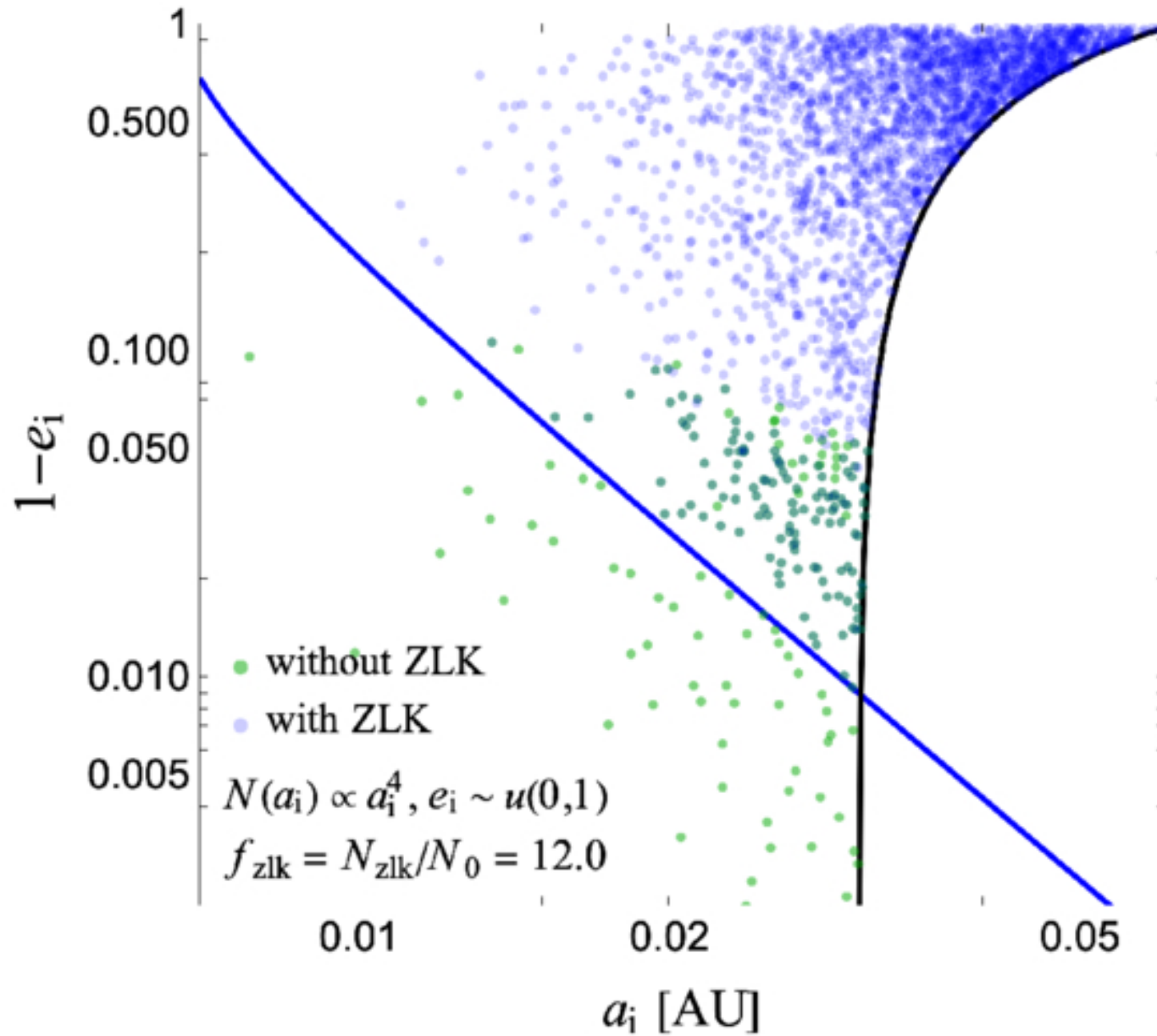
Figure 4. from Wen-Fan Feng et al 2026 Astrophys. J. Lett. 1003 doi:10.3847/2041-8213/ae6b6a https://dx.doi.org/10.3847/2041-8213/ae6b6a © 2026. The Author(s). Published by the American Astronomical Society.
