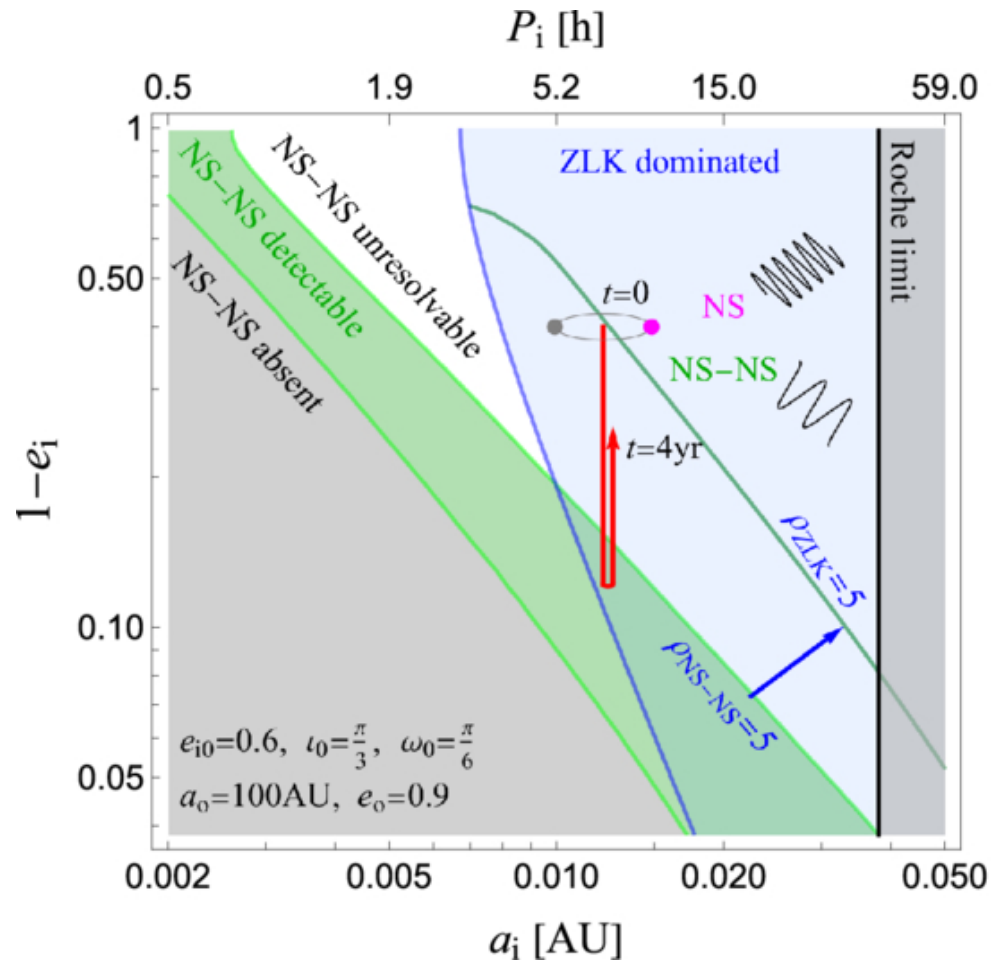
Figure 3. from Wen-Fan Feng et al 2026 Astrophys. J. Lett. 1003 doi:10.3847/2041-8213/ae6b6a https://dx.doi.org/10.3847/2041-8213/ae6b6a © 2026. The Author(s). Published by the American Astronomical Society.
