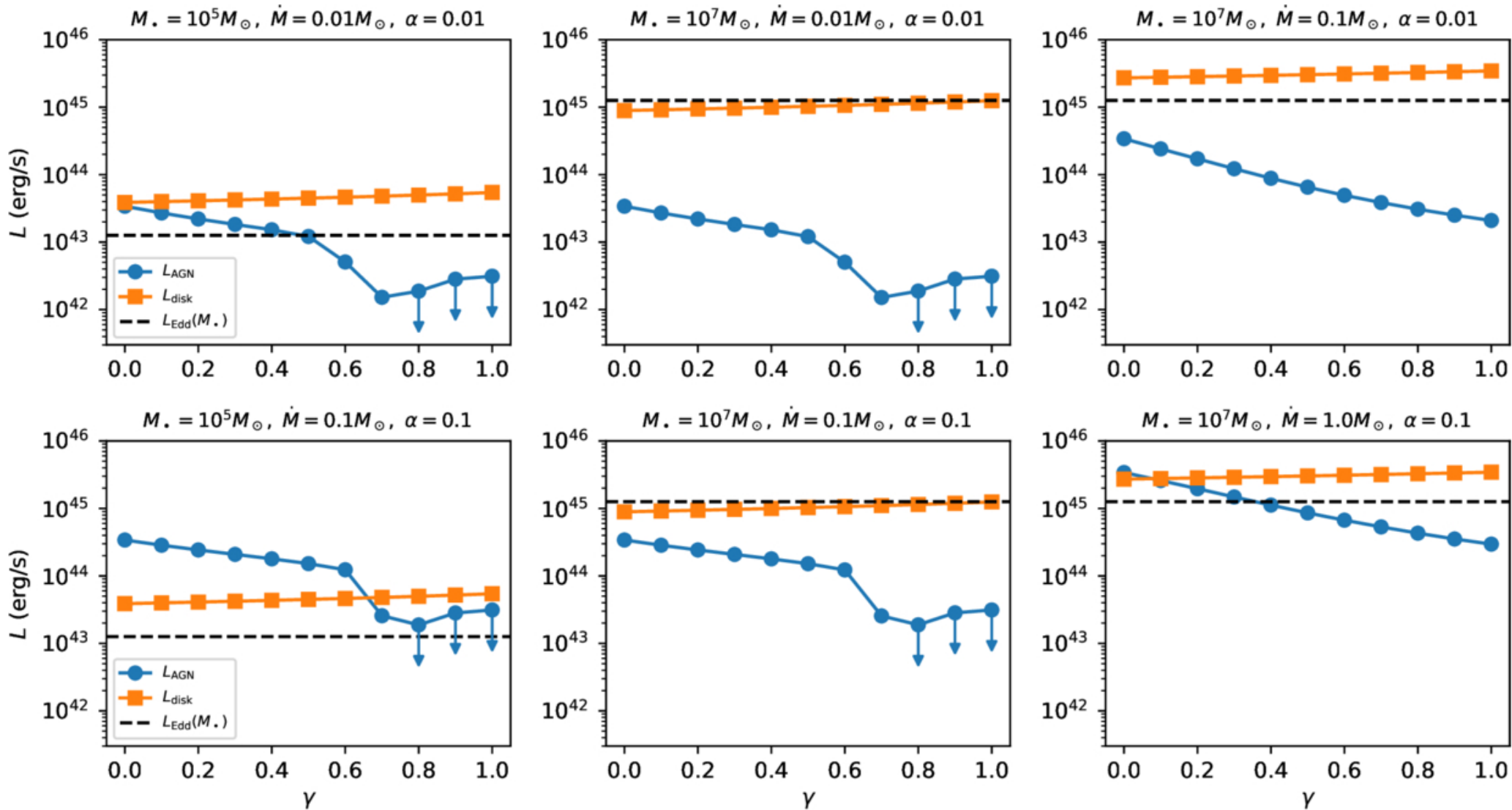
Figure 6. from Yi-Xian Chen et al 2026 Astrophys. J. Lett. 1003 doi:10.3847/2041-8213/ae6b69 https://dx.doi.org/10.3847/2041-8213/ae6b69 © 2026. The Author(s). Published by the American Astronomical Society.
