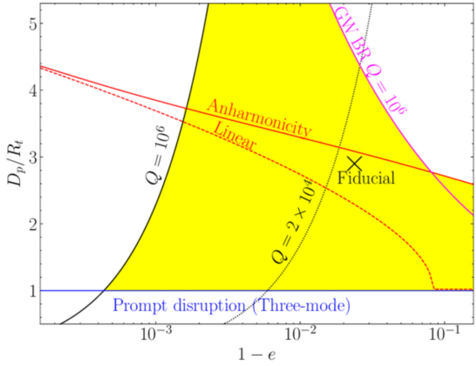
Figure 3. from Shu Yan Lau et al 2026 Astrophys. J. Lett. 1003 doi:10.3847/2041-8213/ae6b68 https://dx.doi.org/10.3847/2041-8213/ae6b68 © 2026. The Author(s). Published by the American Astronomical Society.
