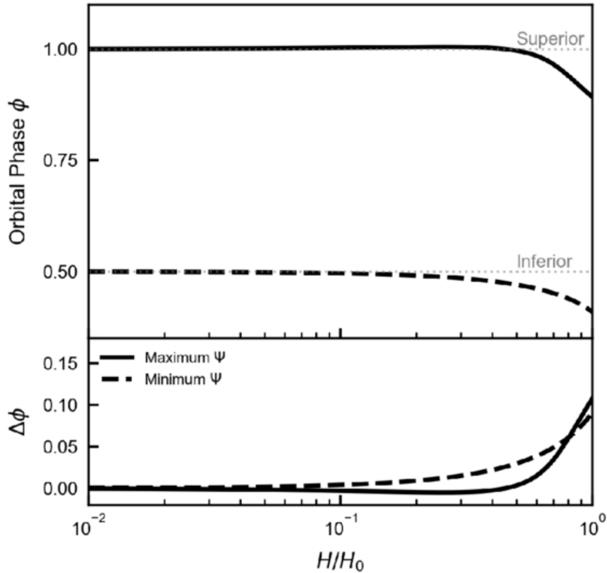
Figure C1. from Xing-Fu Zhang et al 2026 Astrophys. J. Lett. 1003 doi:10.3847/2041-8213/ae6a9d https://dx.doi.org/10.3847/2041-8213/ae6a9d © 2026. The Author(s). Published by the American Astronomical Society.
