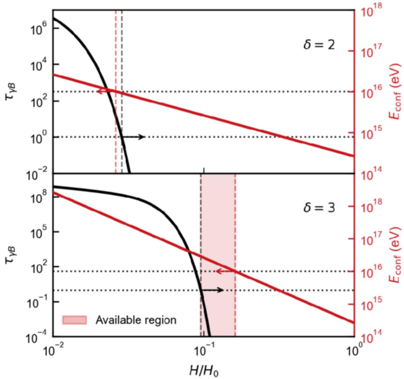
Figure 4. from Xing-Fu Zhang et al 2026 Astrophys. J. Lett. 1003 doi:10.3847/2041-8213/ae6a9d https://dx.doi.org/10.3847/2041-8213/ae6a9d © 2026. The Author(s). Published by the American Astronomical Society.
