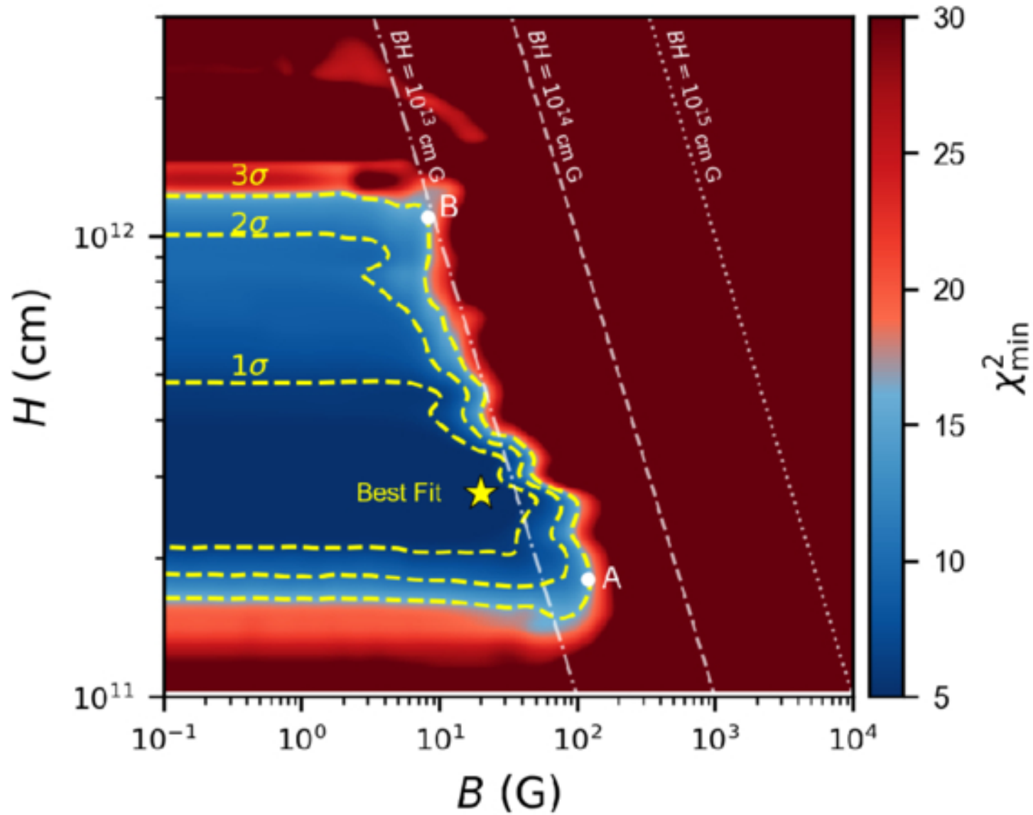
Figure 3. from Xing-Fu Zhang et al 2026 Astrophys. J. Lett. 1003 doi:10.3847/2041-8213/ae6a9d https://dx.doi.org/10.3847/2041-8213/ae6a9d © 2026. The Author(s). Published by the American Astronomical Society.
