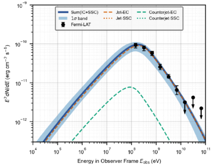
Figure 2. from Xing-Fu Zhang et al 2026 Astrophys. J. Lett. 1003 doi:10.3847/2041-8213/ae6a9d https://dx.doi.org/10.3847/2041-8213/ae6a9d © 2026. The Author(s). Published by the American Astronomical Society.
