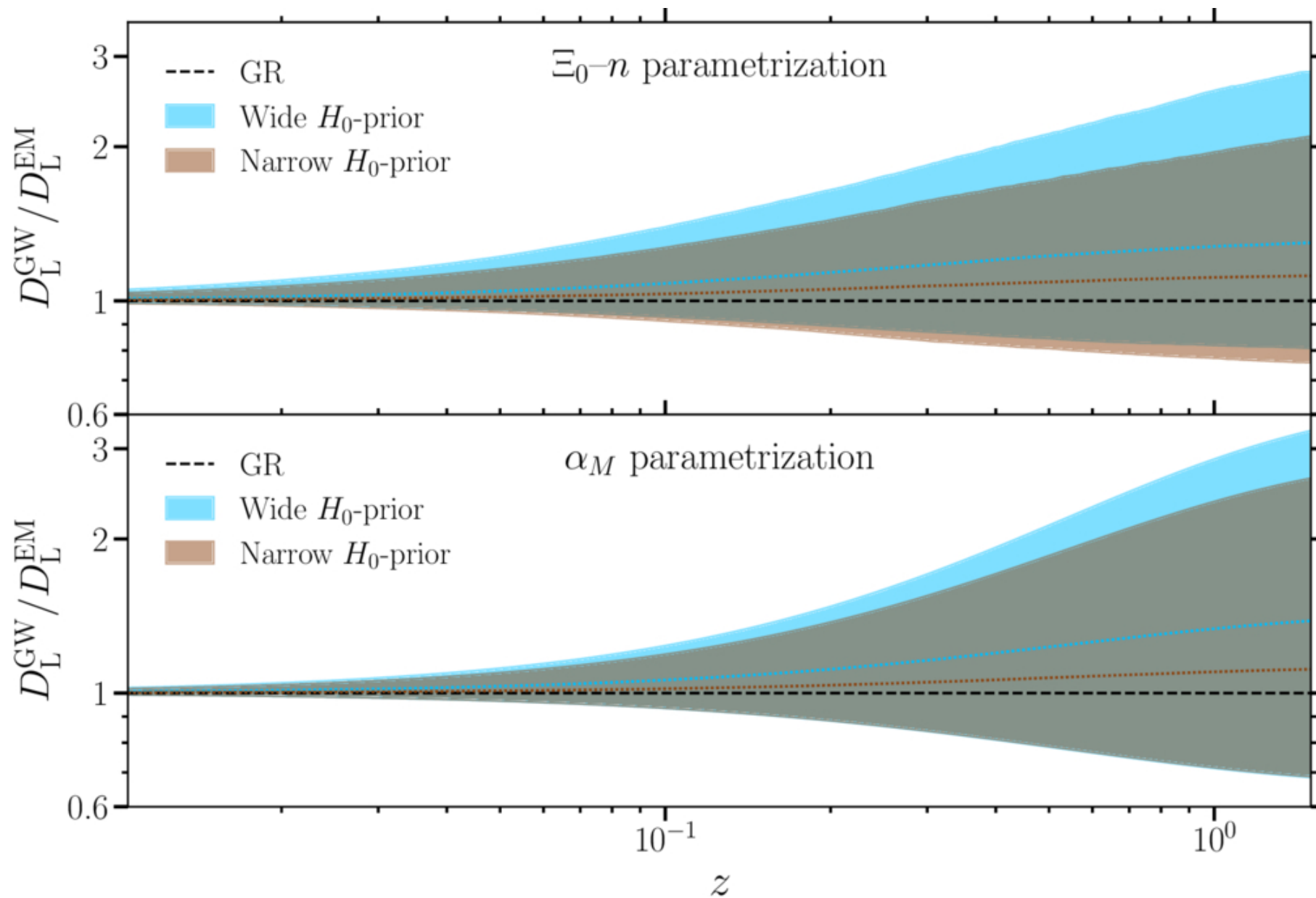
Figure 9. from A. G. Abac et al 2026 Astrophys. J. Lett. 1007 doi:10.3847/2041-8213/ae69dd https://dx.doi.org/10.3847/2041-8213/ae69dd © 2026. The Author(s). Published by the American Astronomical Society.
