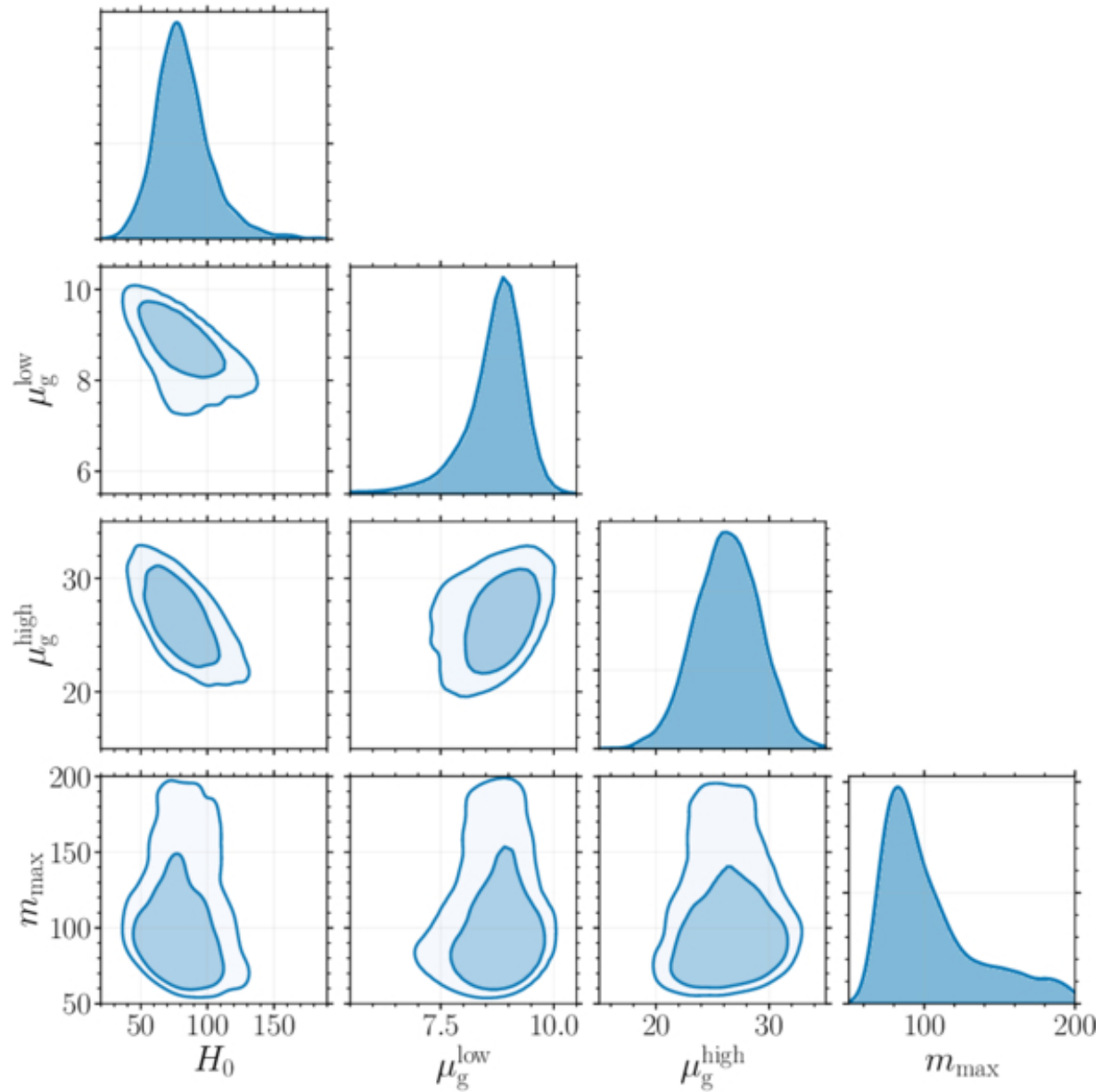
Figure 7. from A. G. Abac et al 2026 Astrophys. J. Lett. 1007 doi:10.3847/2041-8213/ae69dd https://dx.doi.org/10.3847/2041-8213/ae69dd © 2026. The Author(s). Published by the American Astronomical Society.
