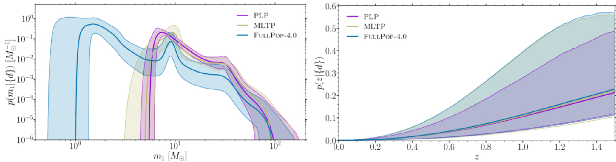
Figure 6. from A. G. Abac et al 2026 Astrophys. J. Lett. 1007 doi:10.3847/2041-8213/ae69dd https://dx.doi.org/10.3847/2041-8213/ae69dd © 2026. The Author(s). Published by the American Astronomical Society.
