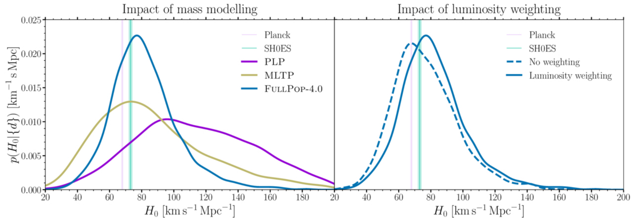
Figure 5. from A. G. Abac et al 2026 Astrophys. J. Lett. 1007 doi:10.3847/2041-8213/ae69dd https://dx.doi.org/10.3847/2041-8213/ae69dd © 2026. The Author(s). Published by the American Astronomical Society.
