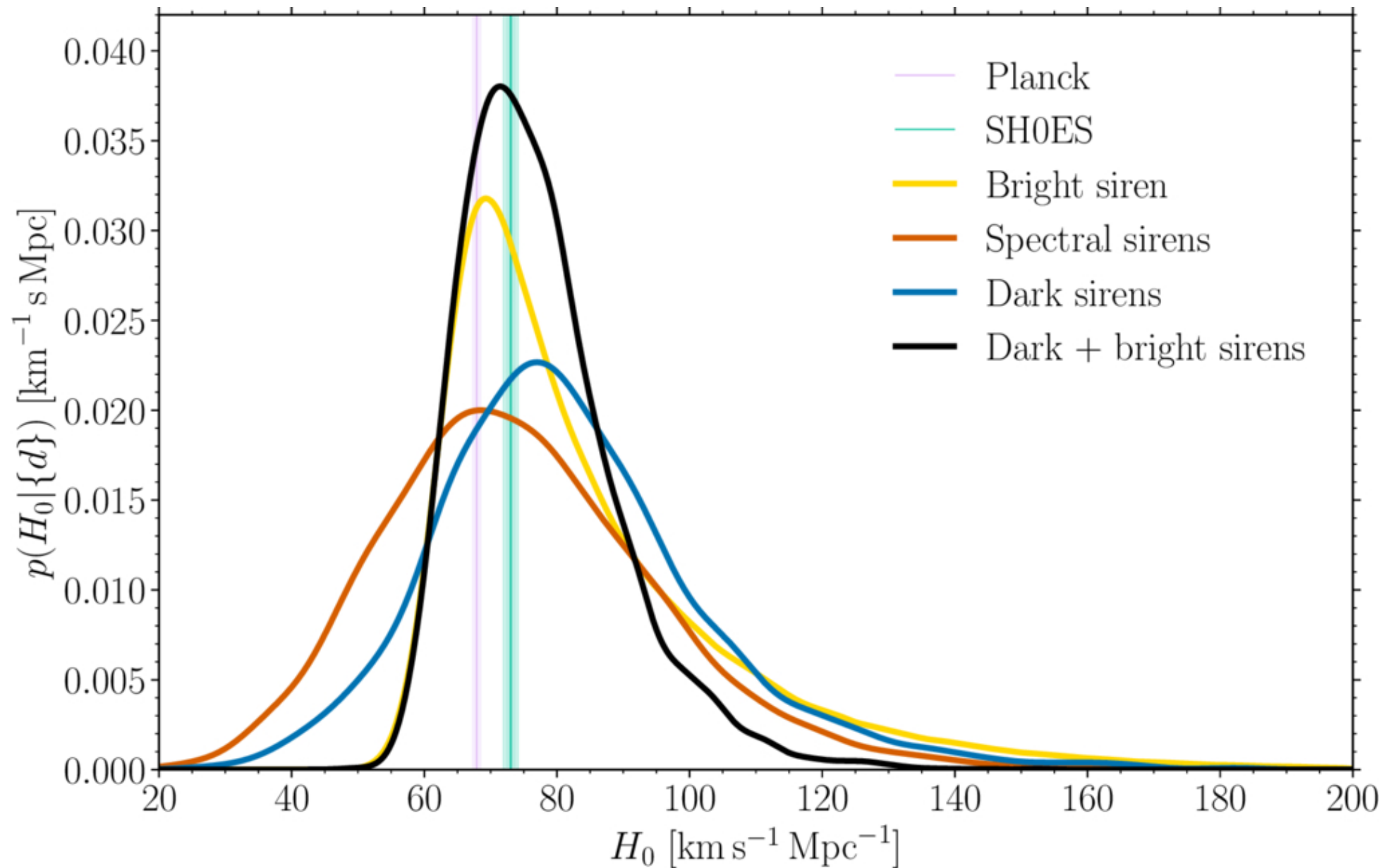
Figure 4. from A. G. Abac et al 2026 Astrophys. J. Lett. 1007 doi:10.3847/2041-8213/ae69dd https://dx.doi.org/10.3847/2041-8213/ae69dd © 2026. The Author(s). Published by the American Astronomical Society.
