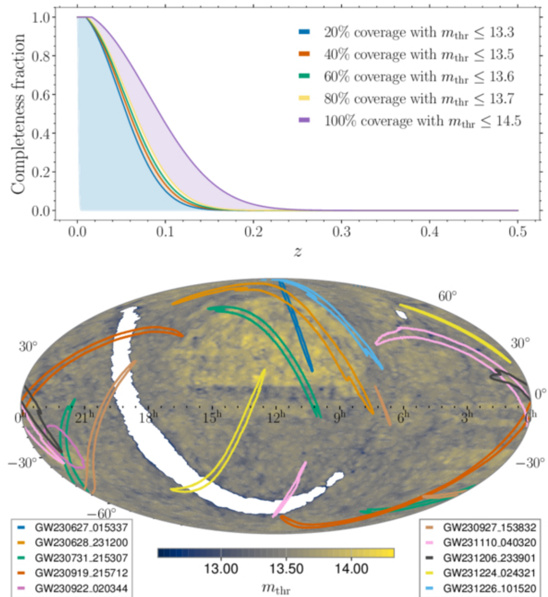
Figure 3. from A. G. Abac et al 2026 Astrophys. J. Lett. 1007 doi:10.3847/2041-8213/ae69dd https://dx.doi.org/10.3847/2041-8213/ae69dd © 2026. The Author(s). Published by the American Astronomical Society.
