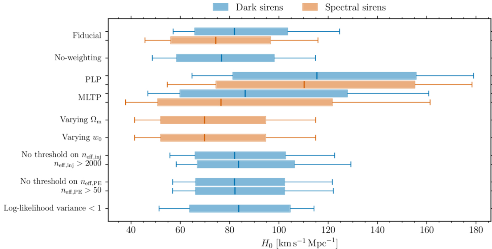
Figure 10. from A. G. Abac et al 2026 Astrophys. J. Lett. 1007 doi:10.3847/2041-8213/ae69dd https://dx.doi.org/10.3847/2041-8213/ae69dd © 2026. The Author(s). Published by the American Astronomical Society.
