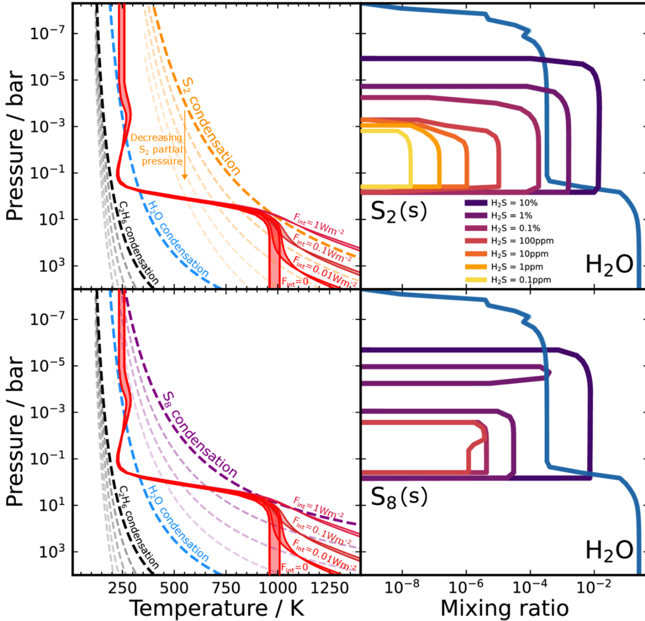
Figure 4. from Sean Jordan et al 2026 Astrophys. J. Lett. 1003 doi:10.3847/2041-8213/ae6864 https://dx.doi.org/10.3847/2041-8213/ae6864 © 2026. The Author(s). Published by the American Astronomical Society.
