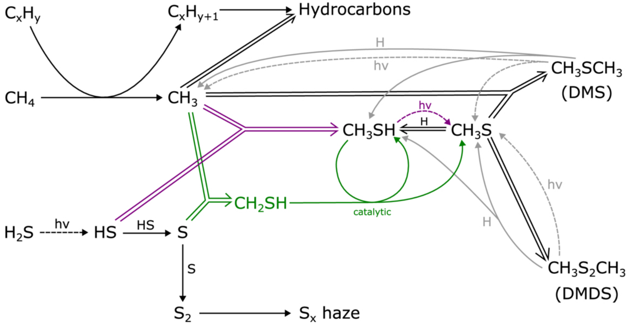
Figure 1. from Sean Jordan et al 2026 Astrophys. J. Lett. 1003 doi:10.3847/2041-8213/ae6864 https://dx.doi.org/10.3847/2041-8213/ae6864 © 2026. The Author(s). Published by the American Astronomical Society.
