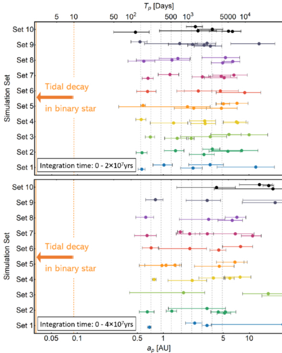
Figure 6. from Bin Liu and Dong Lai 2026 Astrophys. J. Lett. 1003 doi:10.3847/2041-8213/ae6801 https://dx.doi.org/10.3847/2041-8213/ae6801 © 2026. The Author(s). Published by the American Astronomical Society.
