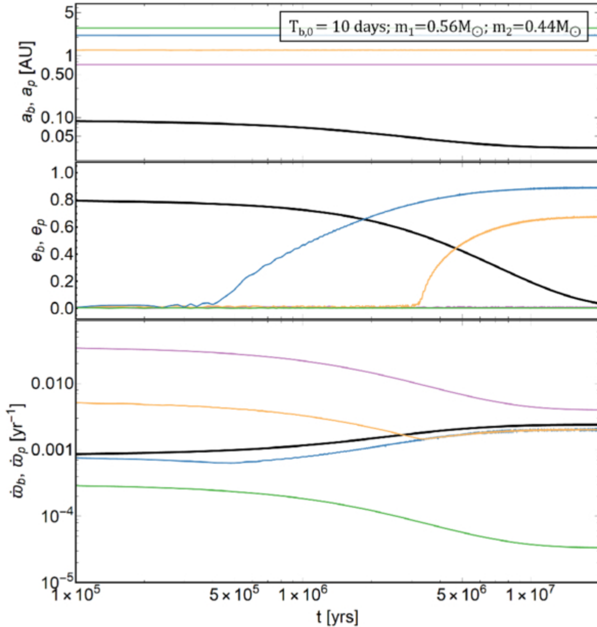
Figure 1. from Bin Liu and Dong Lai 2026 Astrophys. J. Lett. 1003 doi:10.3847/2041-8213/ae6801 https://dx.doi.org/10.3847/2041-8213/ae6801 © 2026. The Author(s). Published by the American Astronomical Society.
